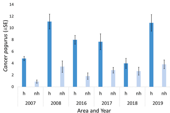
Fig. 7. Average number of Cancer pagurus ( \pm SE) comparing complex foundations with holes (h) and non-complex foundations with no holes (nh) for all years.
